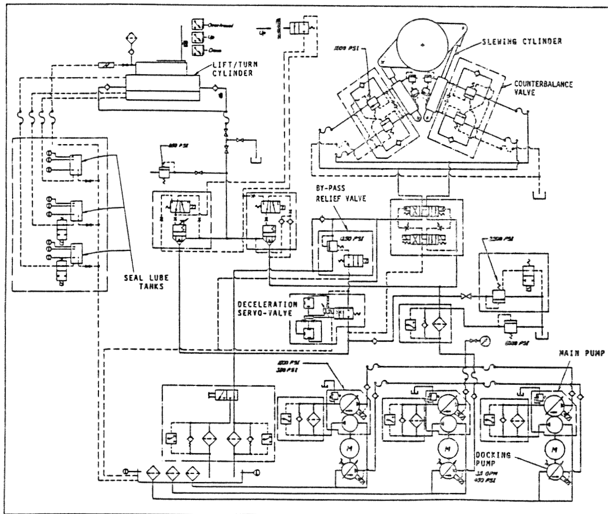
FIGURE 4 - PIER HYDRAULIC SCHEMATIC
