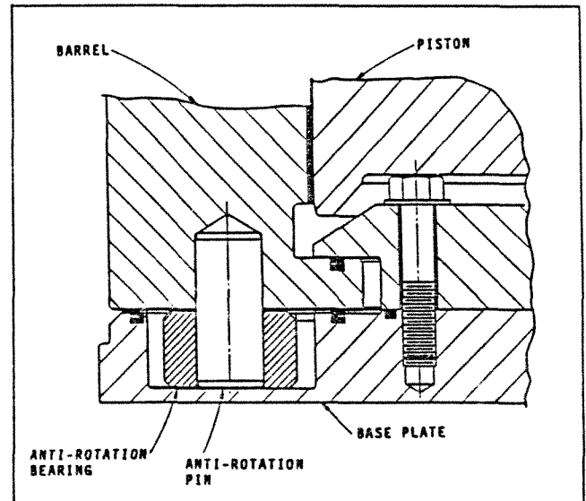
BARREL ANTI-ROTATION PIN AND BEARING
