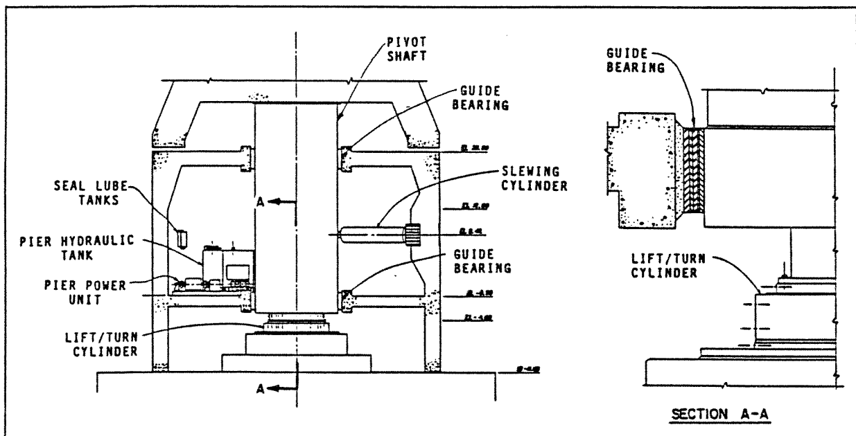
FIGURE 5 - LIFT/TURN CYLINDER AND BEARING LOCATIONS
