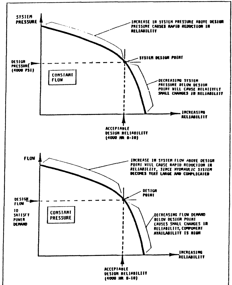
FIGURE 11 - HYDRAULIC SYSTEM RELIABILITY
