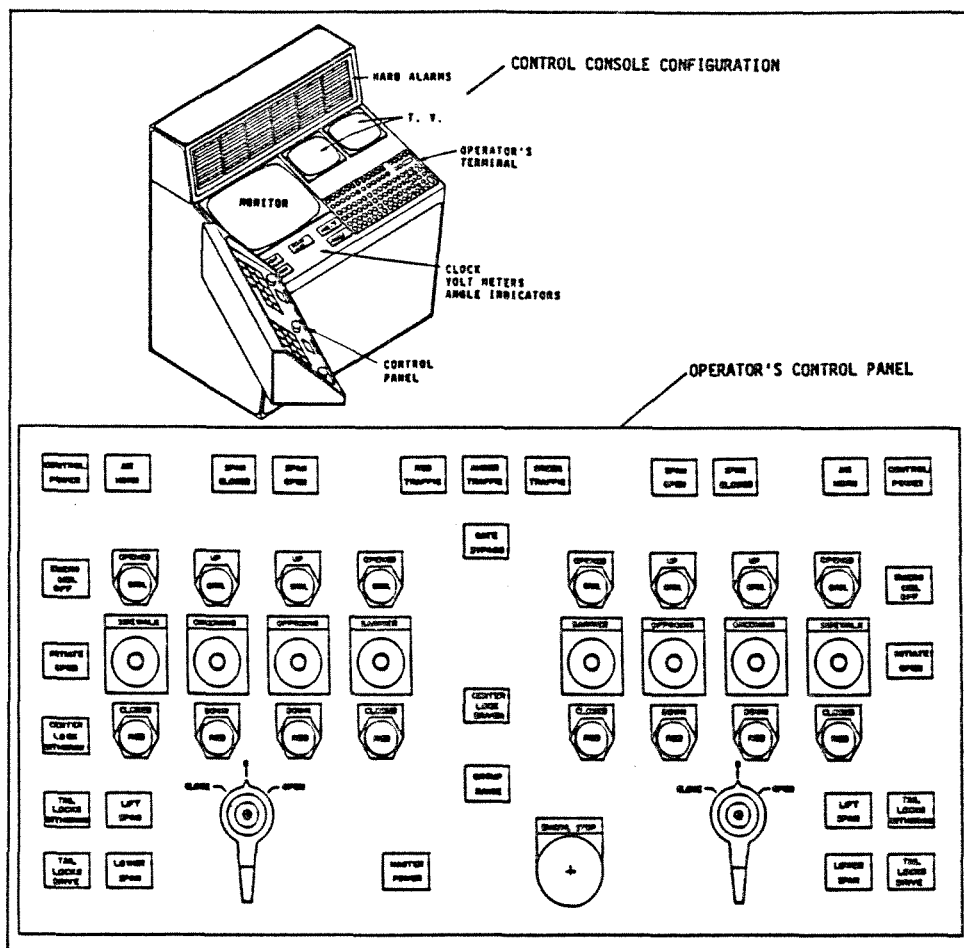
FIGURE 3 - CONTROL CONSOLE CONFIGURATION
