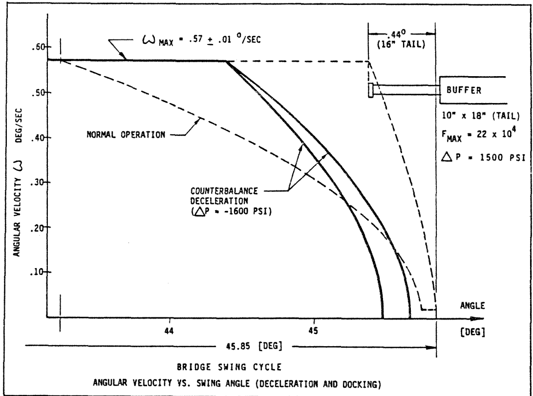
FIGURE 10 - ANGULAR VELOCITY VS. SWING ANGLE - DECELERATION AND DOCKING
