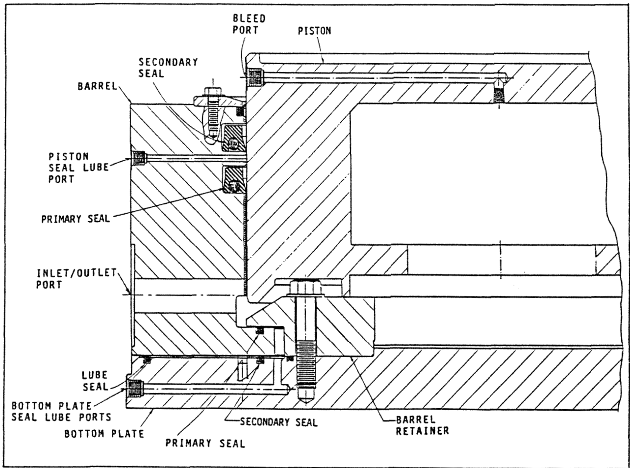
FIGURE 6 - LIFT/TURN CYLINDER HALF SECTION
