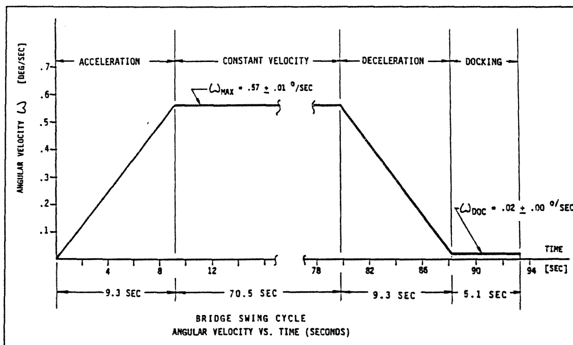
FIGURE 9 - ANGULAR VELOCITY VS. TIME
