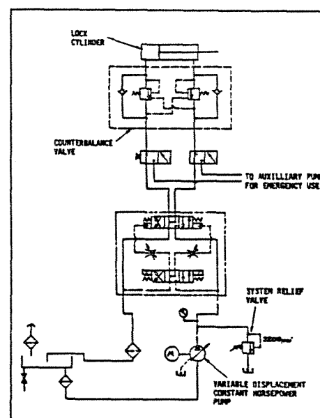
FIGURE 8 - LOCKS HYDRAULIC SCHEMATIC
